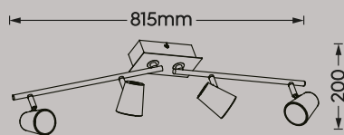
Strahler · Spot incl. SMD-LED 4 x 6,5 W / 4 x 600 Lumen 3.000 Kelvin 873110431
