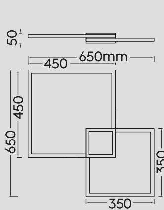
Deckenleuchte · Ceiling lamp incl. SMD-LED 28 W / 3.200 Lumen 4.000 Kelvin 676240331
